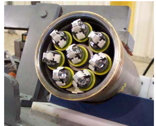
155mm, M864 DPICM
